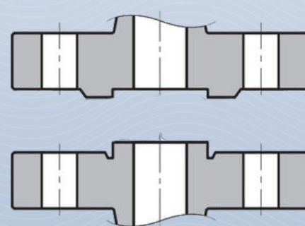
TYPE G AND H - O-RING SPIGOT AND O- GROOVE FACE
