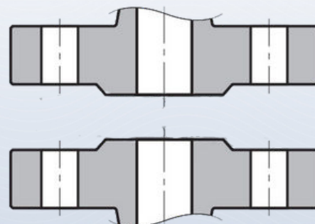
TYPE B - RAISED FACE
