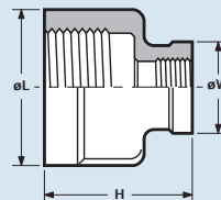
Reducing socket / Reduzier Muffe / Manchon de reduction / Verloop sok
