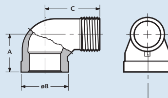
Street elbow F-M / Winkel I-A / Coude F-M / Knie Bi-Bu
