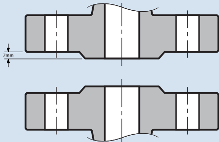
Raised Face (400LBS and up)
