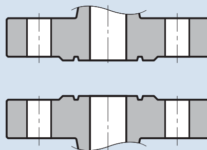
Ring Type Joint Face
