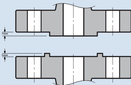
Male and Female Face
